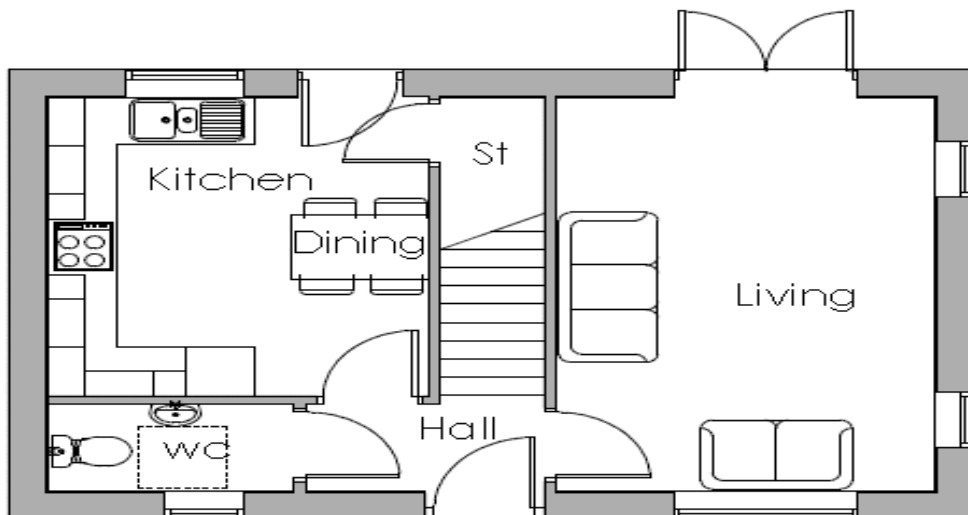
Ground Floor
